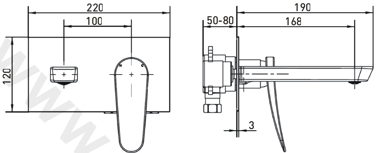
Wall Mounted Bath Filler
